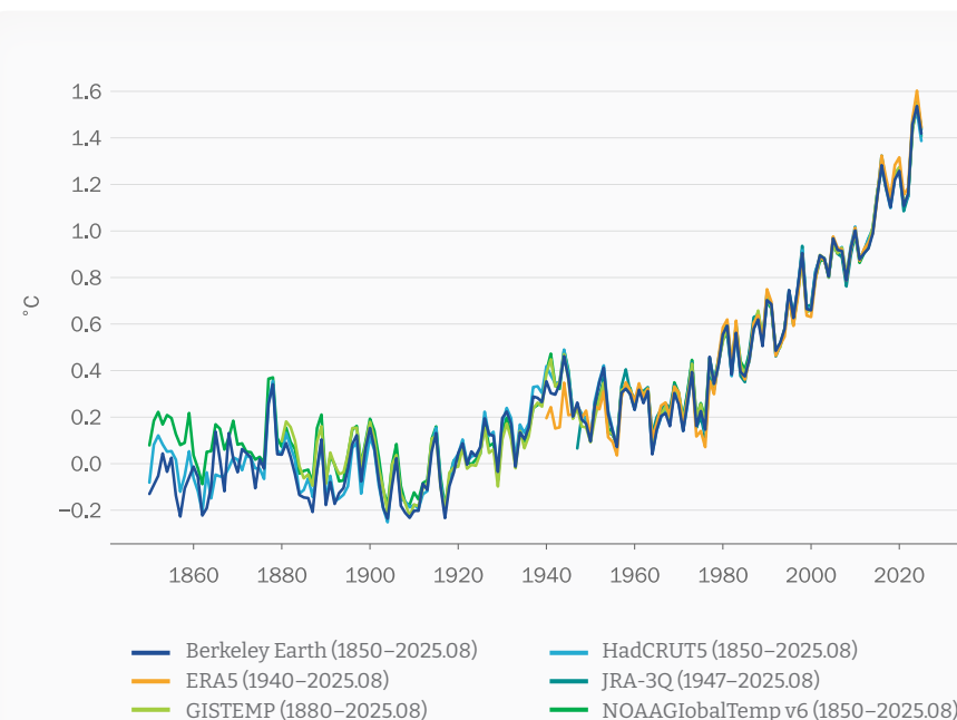
Figure 2. Annual global mean temperature anomalies (relative to 1850–1900) from 1850 to 2025 from six datasets. The 2025 average is based on data from January to August.
