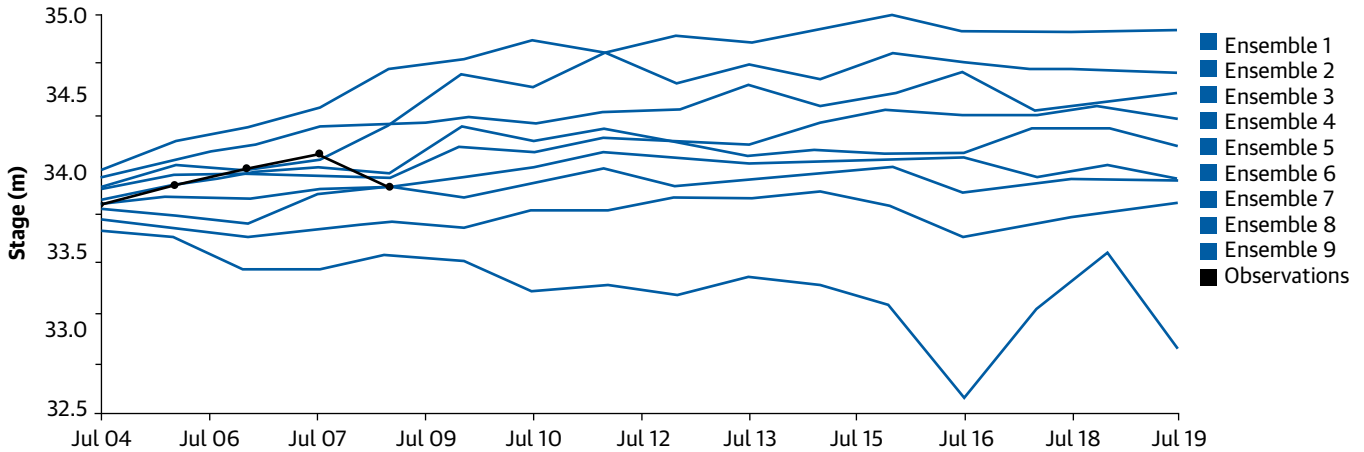
FIGURE 3.2. NCAR Ensemble Flood Forecasted Stage at Baltara
