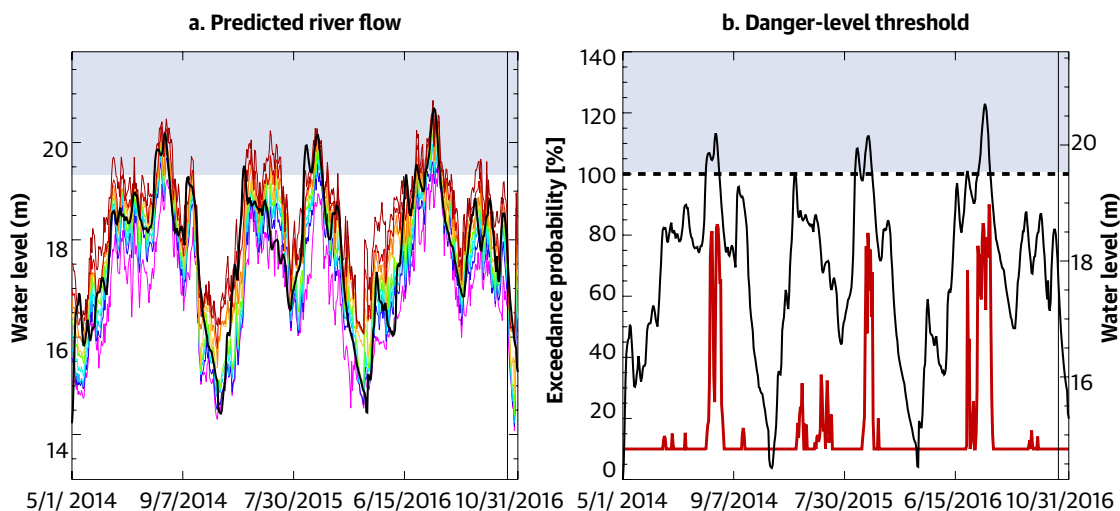
FIGURE 3.3. Forecasts for Bahadurabad (Brahmaputra River) for Three Monsoon Seasons (2014-16)
